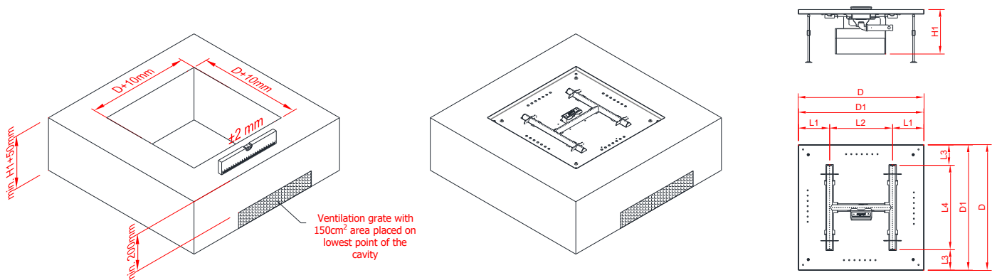
Picture 1 – Cavity size
