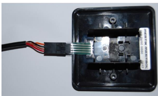
Photo 12 – Wall Switch connection and serial number location
