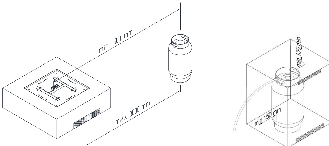
Picture 3 – Gas cylinder distance
