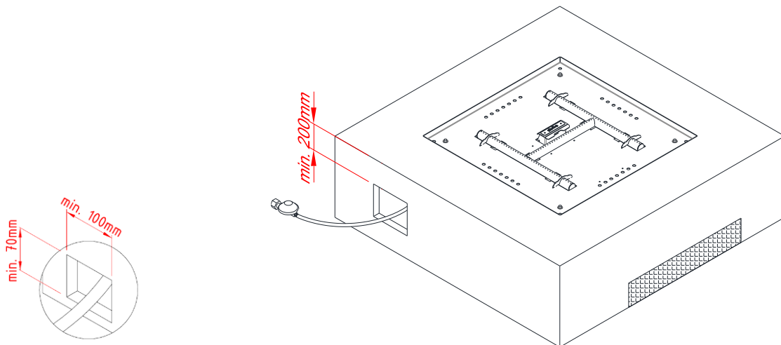
Picture 2 – Gas connection
